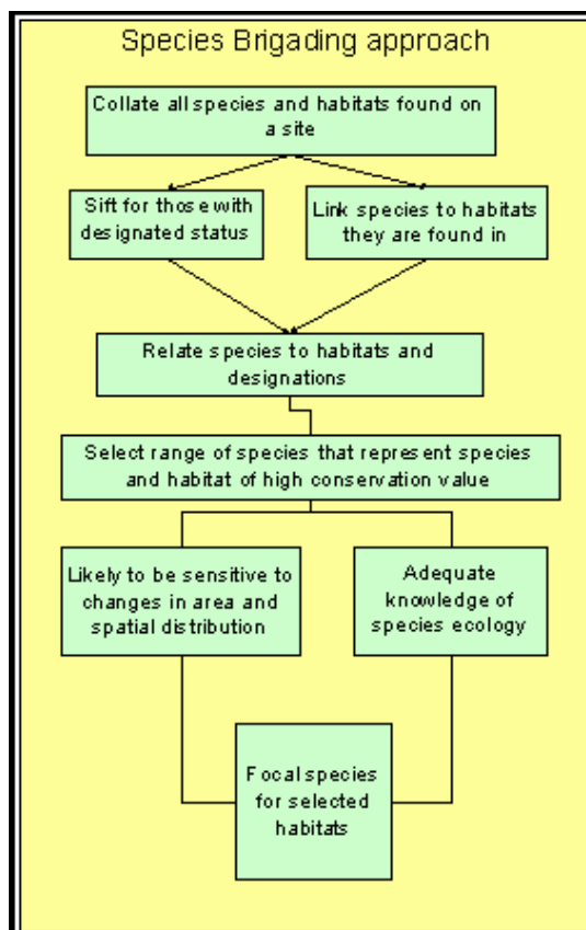
Figure 3 – Focal species selection
